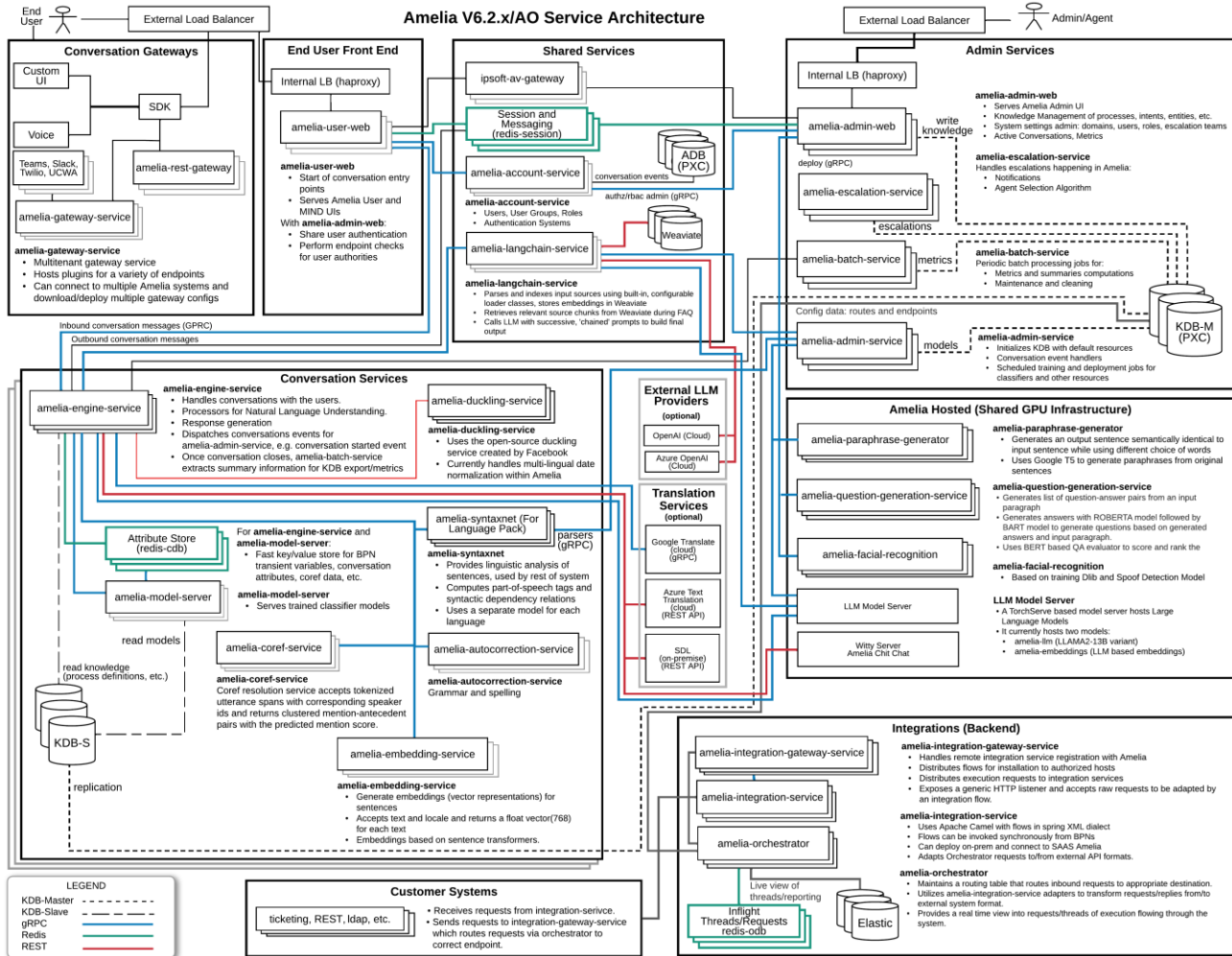
Figure 1. Amelia 6.2.x System Architecture
